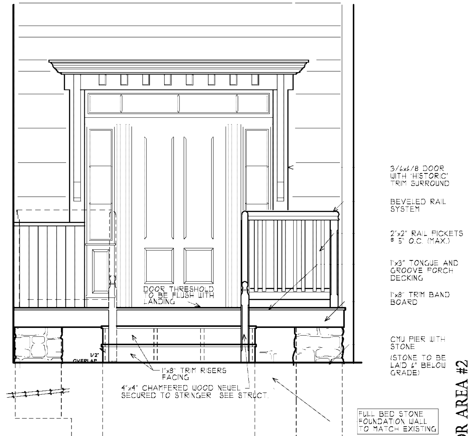
PARTIAL LANDING DOOR AREA #2
