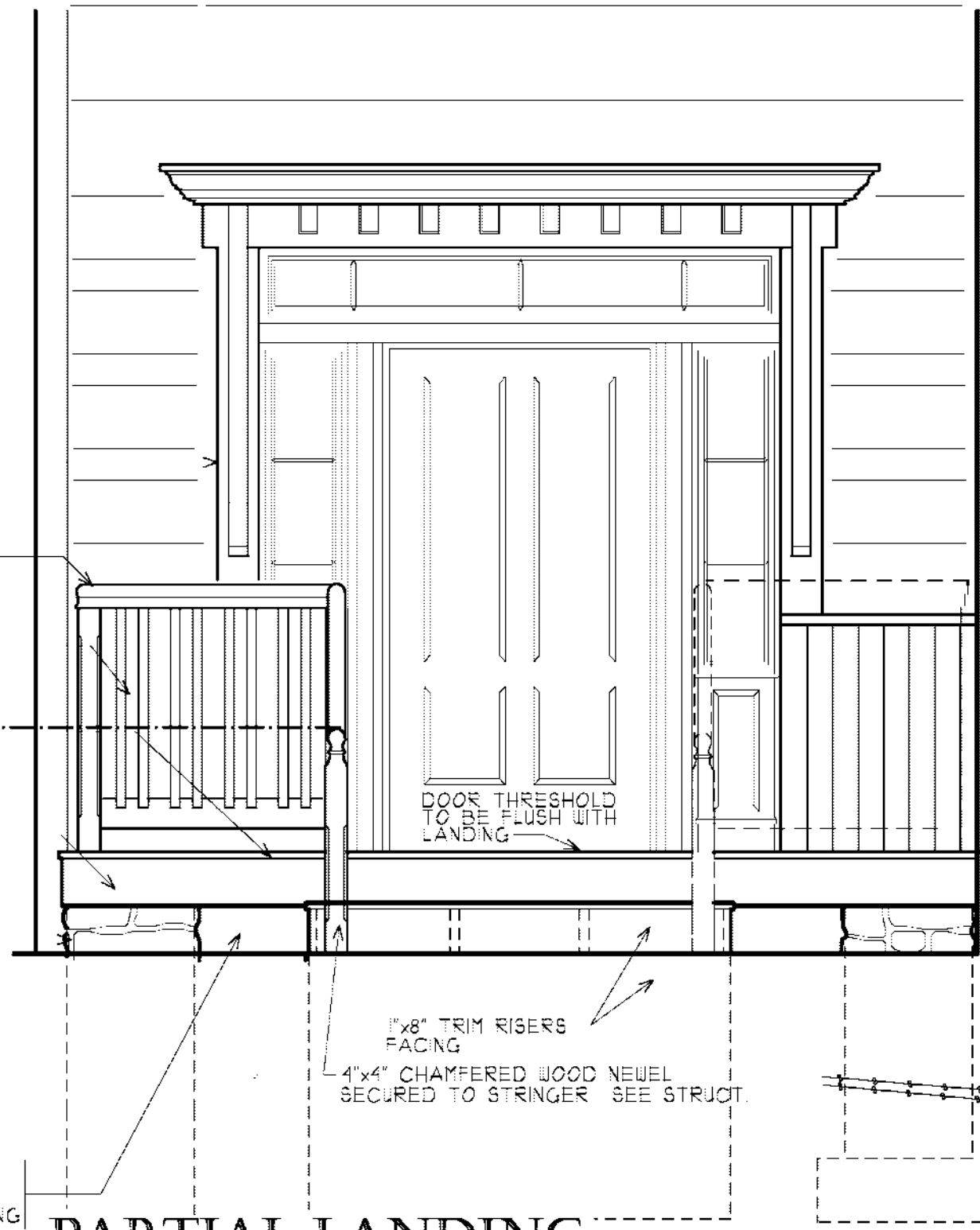
PARTIAL LANDING DOOR AREA #3
