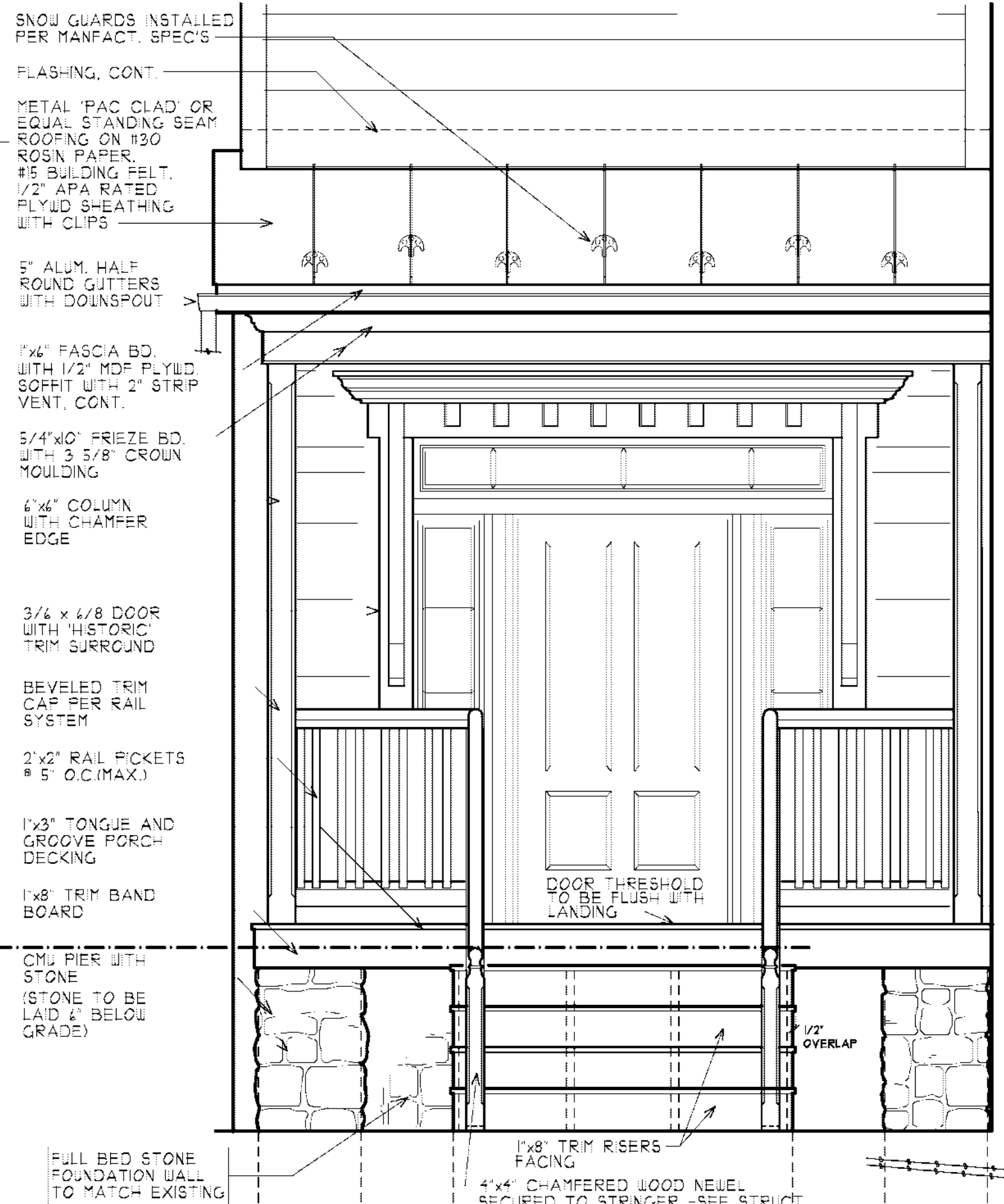
PARTIAL COVERED PORCH ELEV.-DOOR AREA #1
