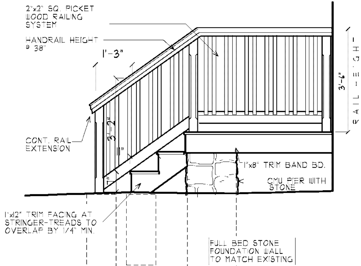
PARTIAL SIDE ELEV. DOOR AREA #2
