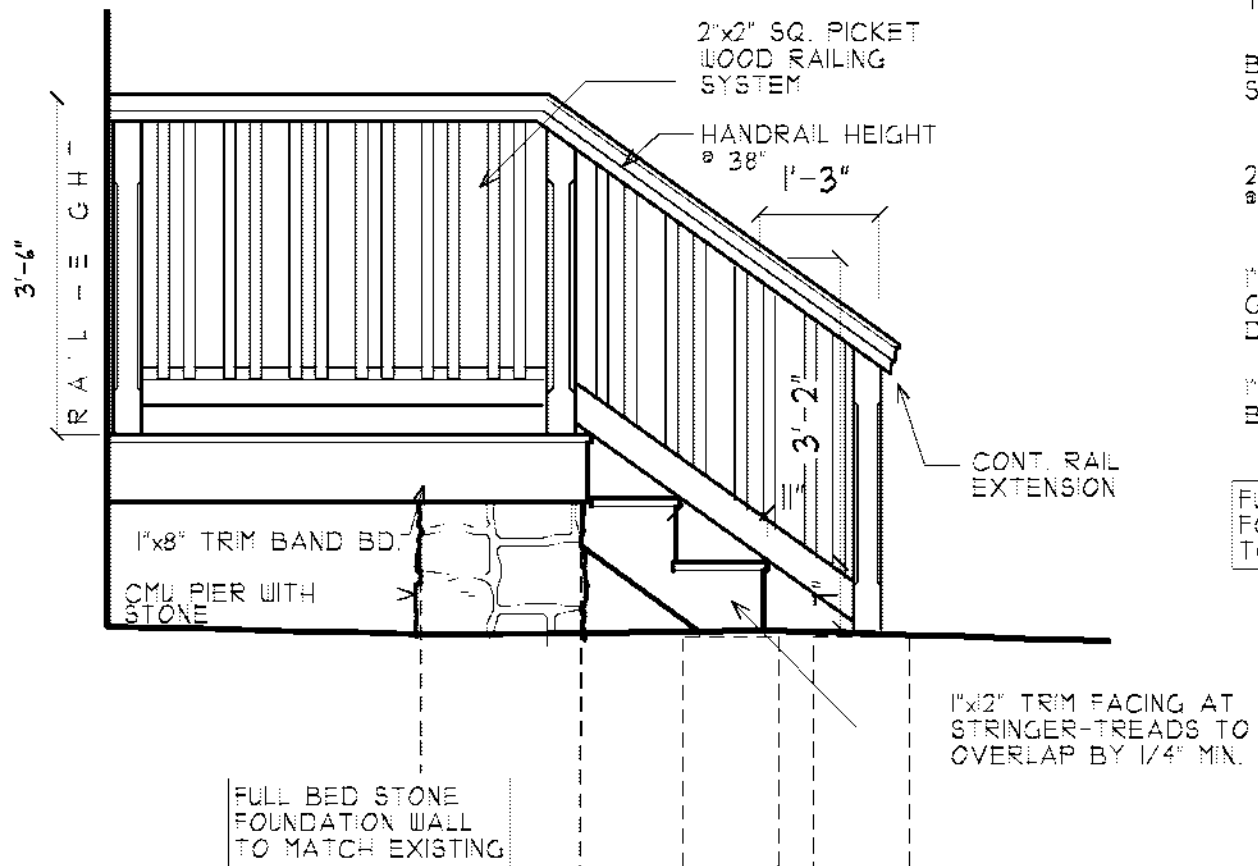
PARTIAL SIDE ELEV. DOOR AREA #4
