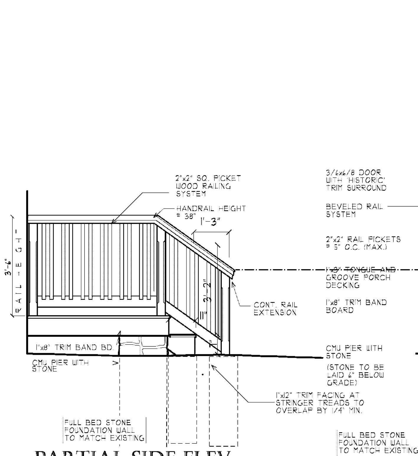
PARTIAL SIDE ELEV. DOOR AREA #3
