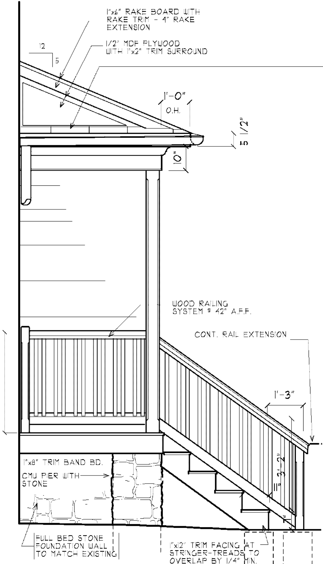
PARTIAL SIDE ELEV. DOOR AREA #1
